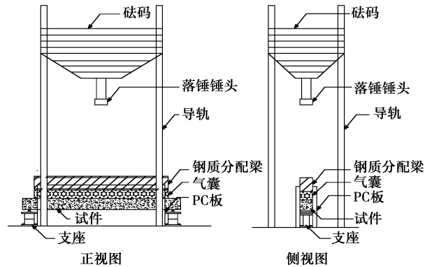
图 1 落锤冲击气囊均布动荷载加载装置 Fig. 1 Drop hammer impacting airbag uniform dynamic loading apparatus
