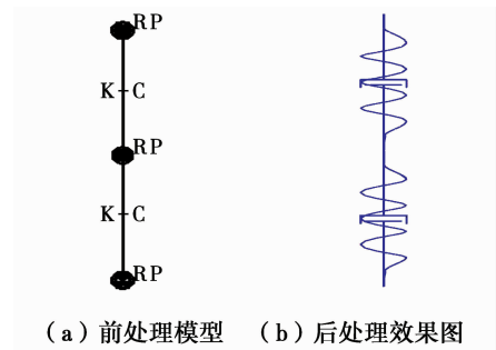
图 3 双自由度弹簧阻尼冲击加载分析模型有限元模型 Fig. 3 Finite element model of two-DOF-Spring-Mass-Dashpot impact loading analytical model
