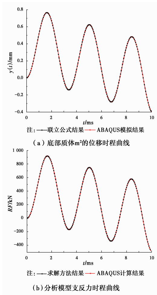
图 4 无阻尼情况下位移和支反力时程曲线 Fig. 4 The y(t) -time curve and RF-time curve without dashpot
