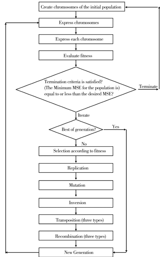
Fig. 2 The procedure of GEP algorithm
