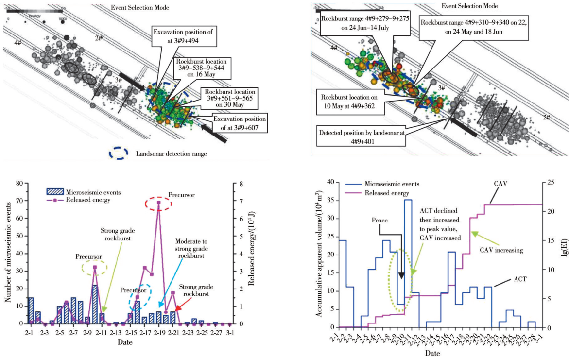
Fig. 6 Data collection of the rockburst events using microseismic systems and some results (Modified after Ma et al. [57])
