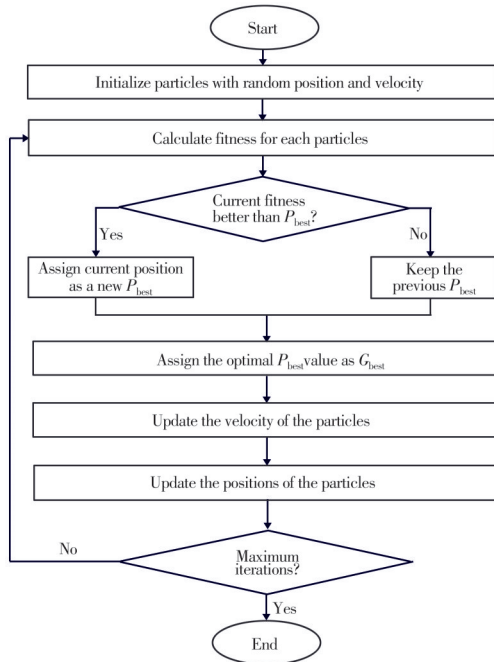
Fig. 4 Optimization procedure of the PSO algorithm
